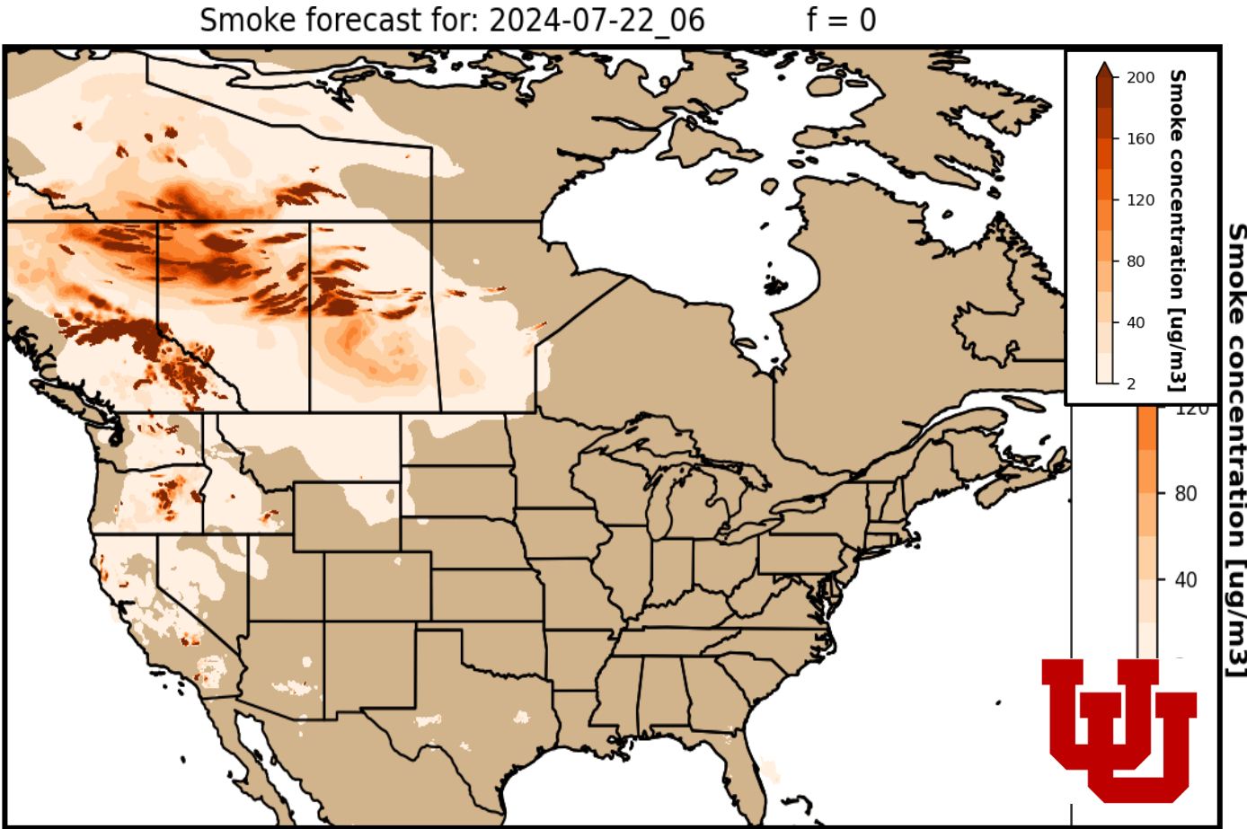
Smoke transport simulated with HYSPLIT-STILT
